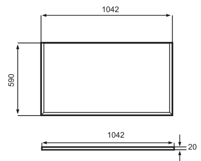
CRYSTAL 1000 SOLID SURFACE TOP 1042x590x20
