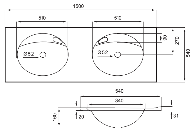
DOUBLE BOWL 1500x540x160
